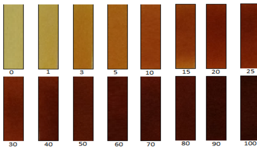
Figure 11. A picrate-paper cyanide color chart for qualitative analysis of CNGs for the range of 0–100 \mu\text{g} \text{CN}^- eq.
