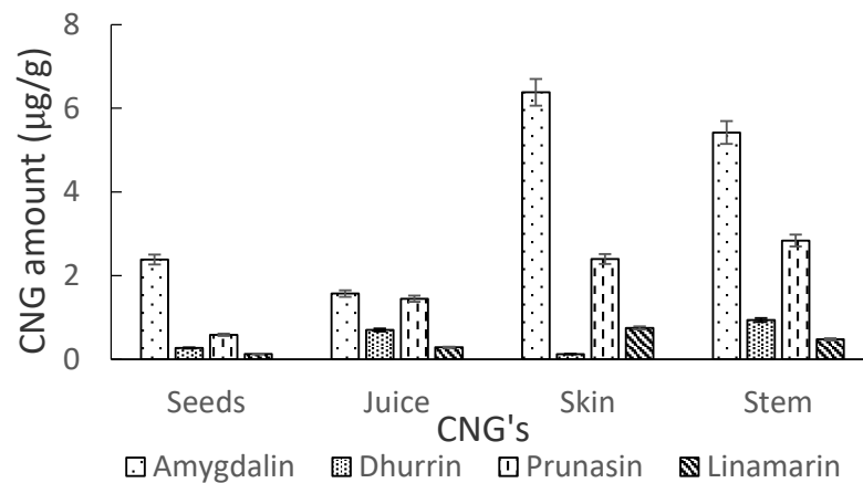
Figure 8. Amounts of CNGs ( \mu\text{g/g} ) in tissues (seeds, juice, skin and stem) of Ozone elderberry samples as measured by UHPLC-MS/MS.
