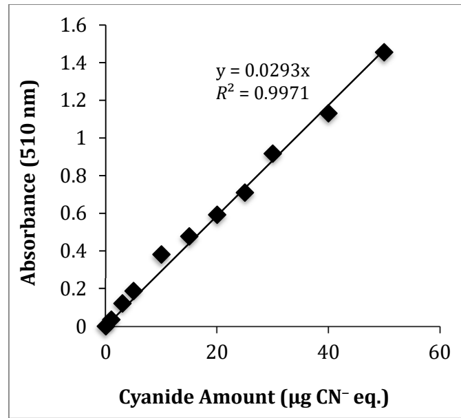
Figure 2. Calibration curve for the amount of CN - eq. produced by reaction of picric acid with HCN using amygdalin as a CNG standard measured by UV-Vis spectrophotometry at \lambda_{\max} = 510 nm.
