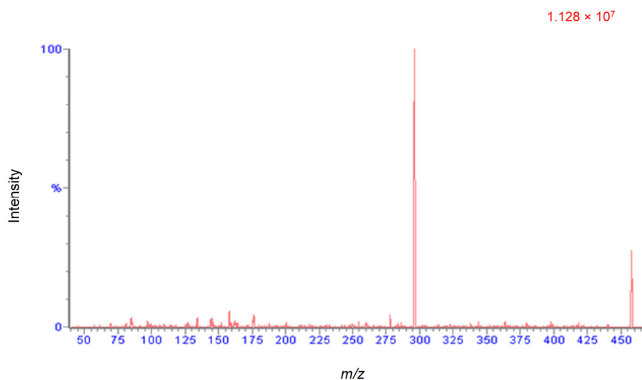
Figure 5. ESI positive mode product ion ( 296\ m/z , product ion) spectrum for amygdalin ( 465\ m/z , precursor ion).
